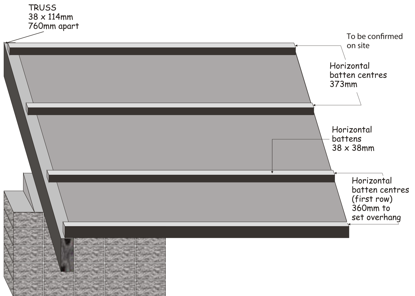
SUGGESTED BATTEN LAYOUT
